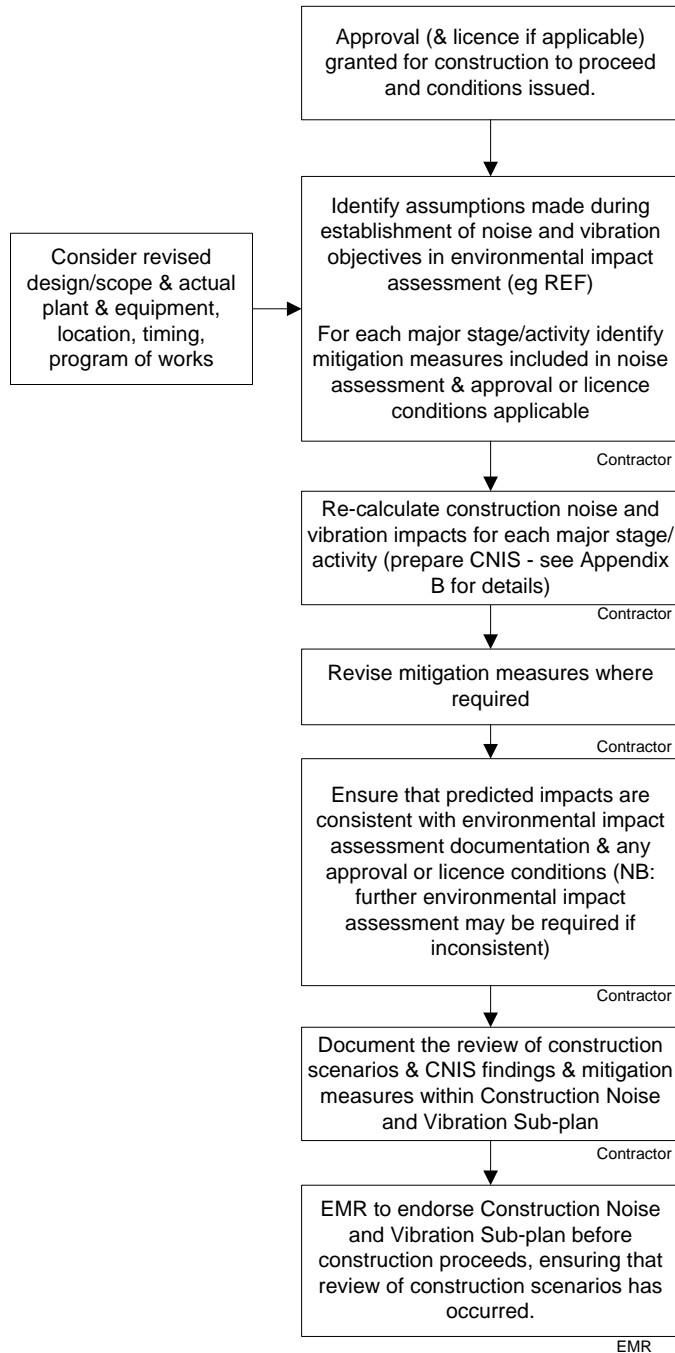
Figure 1: Construction noise and vibration assessment review procedure
