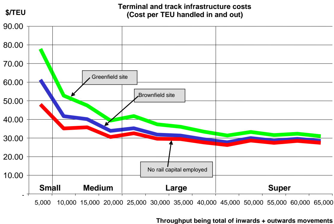
Figure 13 - Indicative terminal unit costs by volume and investment level
