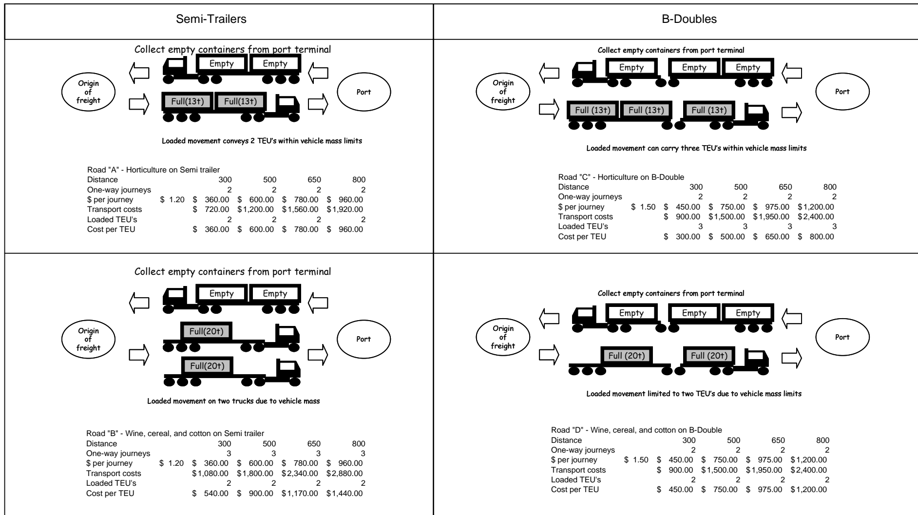
Figure 36 - Typical road vehicle configurations and nominal costs
