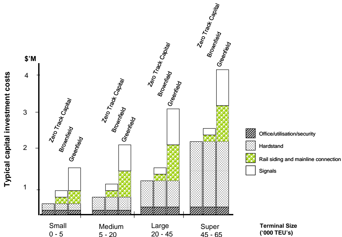
Figure 12 - Estimated capital costs for each investment level and volume consideration
