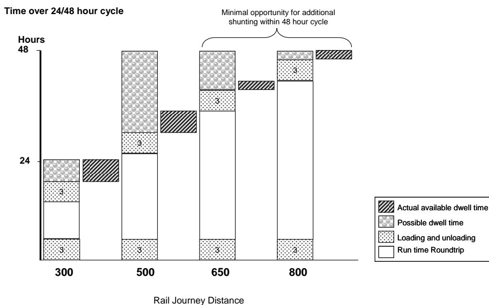
Figure 33 - Relationship between daily train path cycles, and available dwell time
