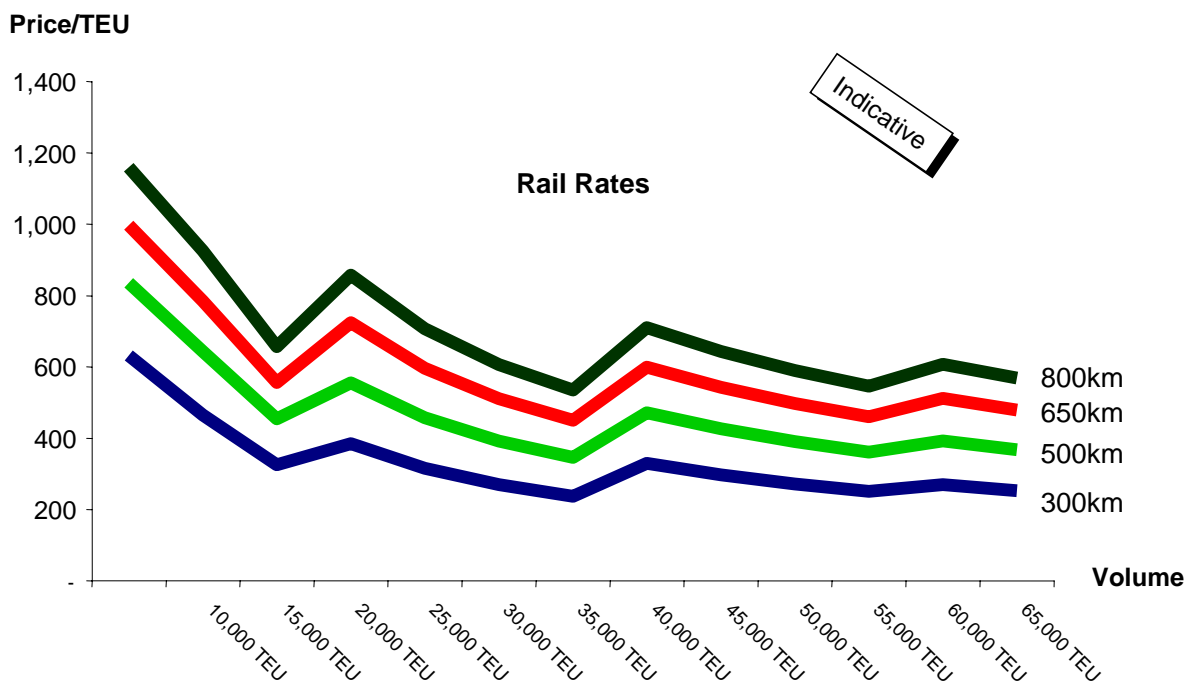
Figure 19 - Average rail-based unit costs for varying volumes and distance to port
