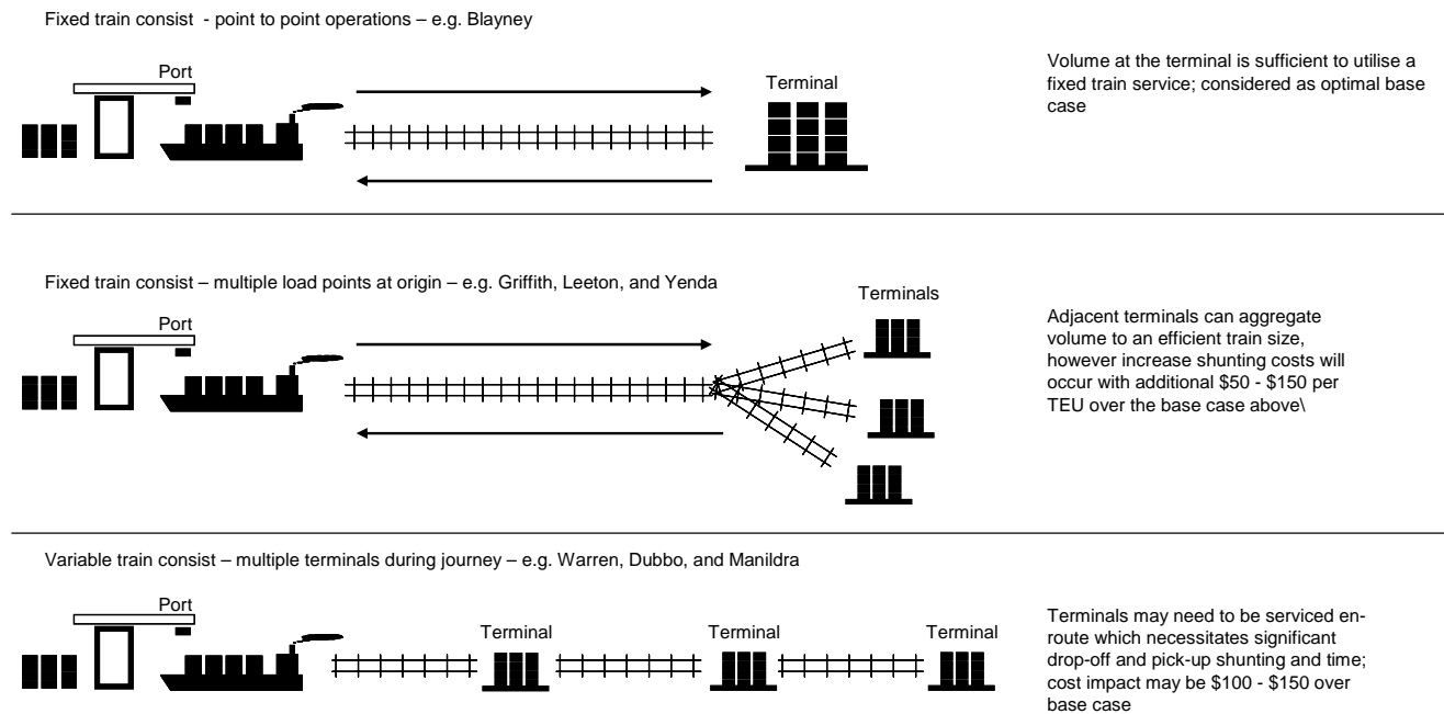
Figure 32 - Various terminal and network configurations
