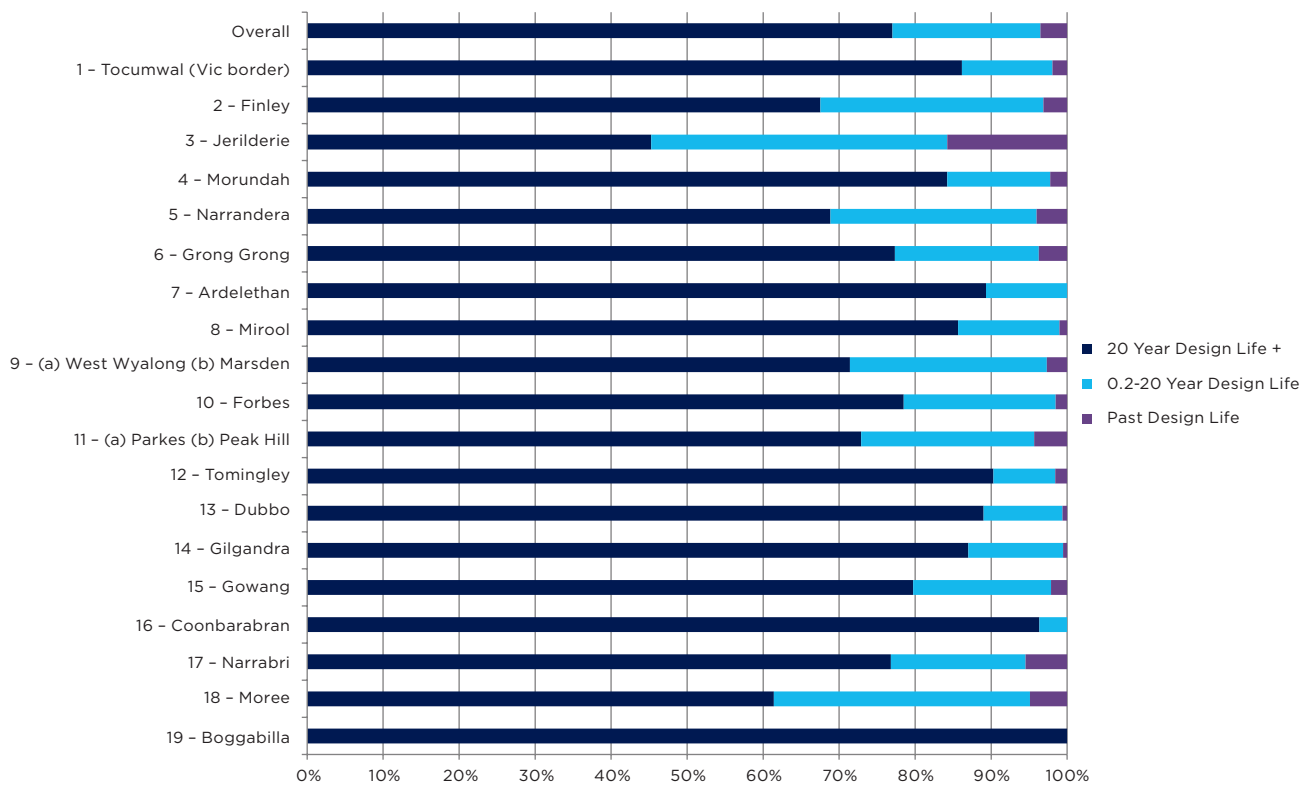
Figure 4.24 Pavement deflection
