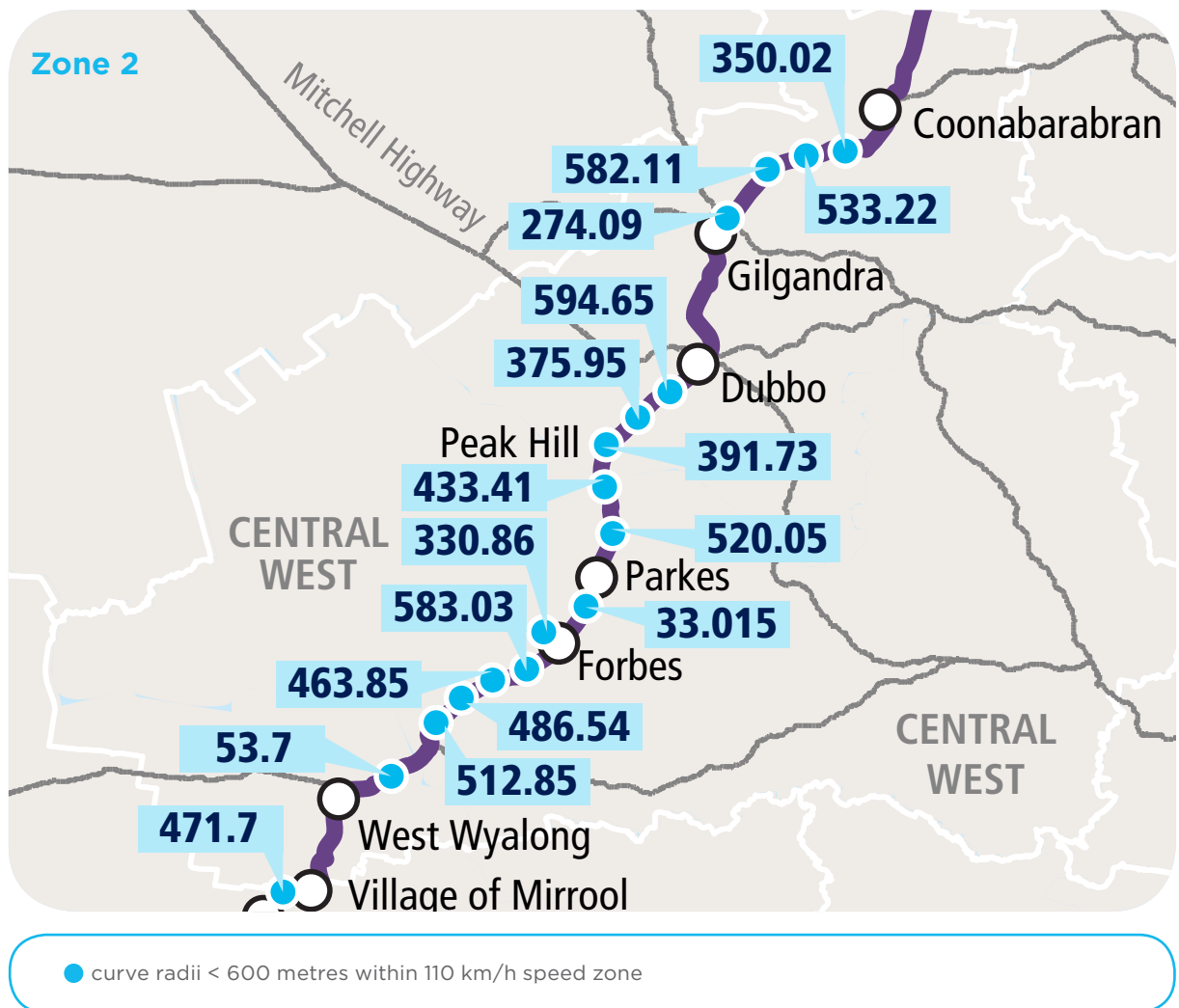
Figure 4.17 Locations where curve radii are less than 600 metres within 110 km/h speed zones (Zone 2)
