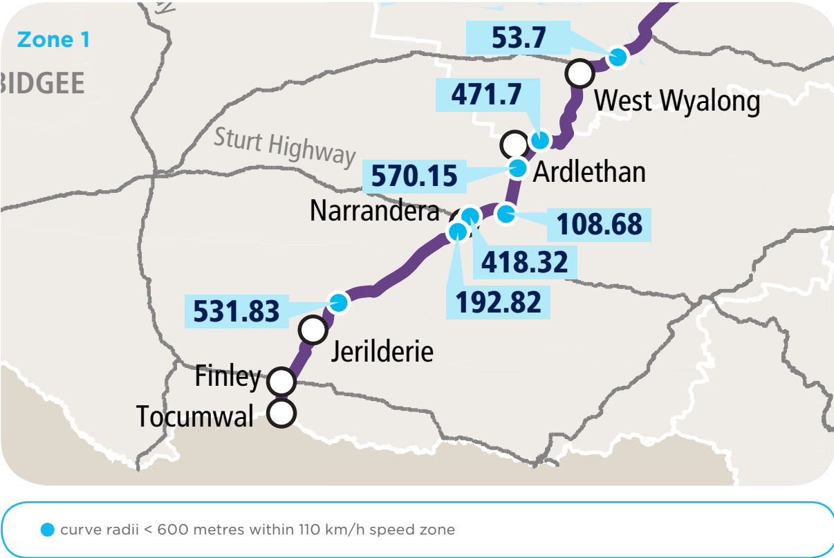
Figure 4.16 Locations where curve radii are less than 600 metres within 110 km/h speed zones (Zone 1)
