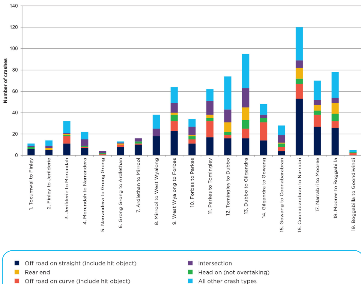
Figure 4.6 Crash types, 2007 to 2011
