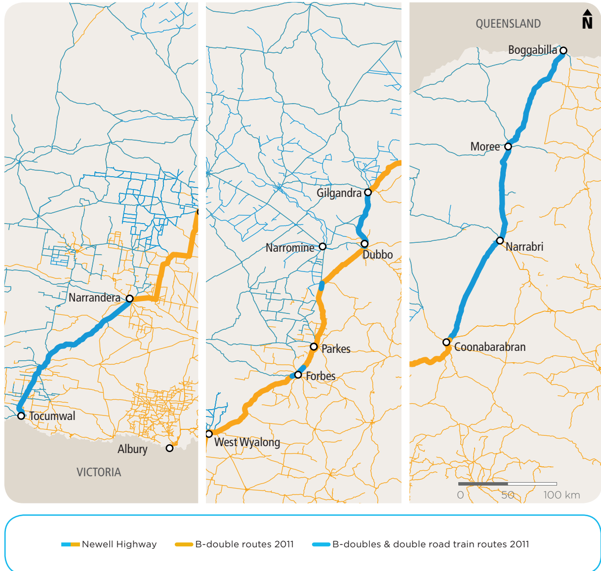
Figure 2.2 Road Train and B-double access along the Newell Highway
