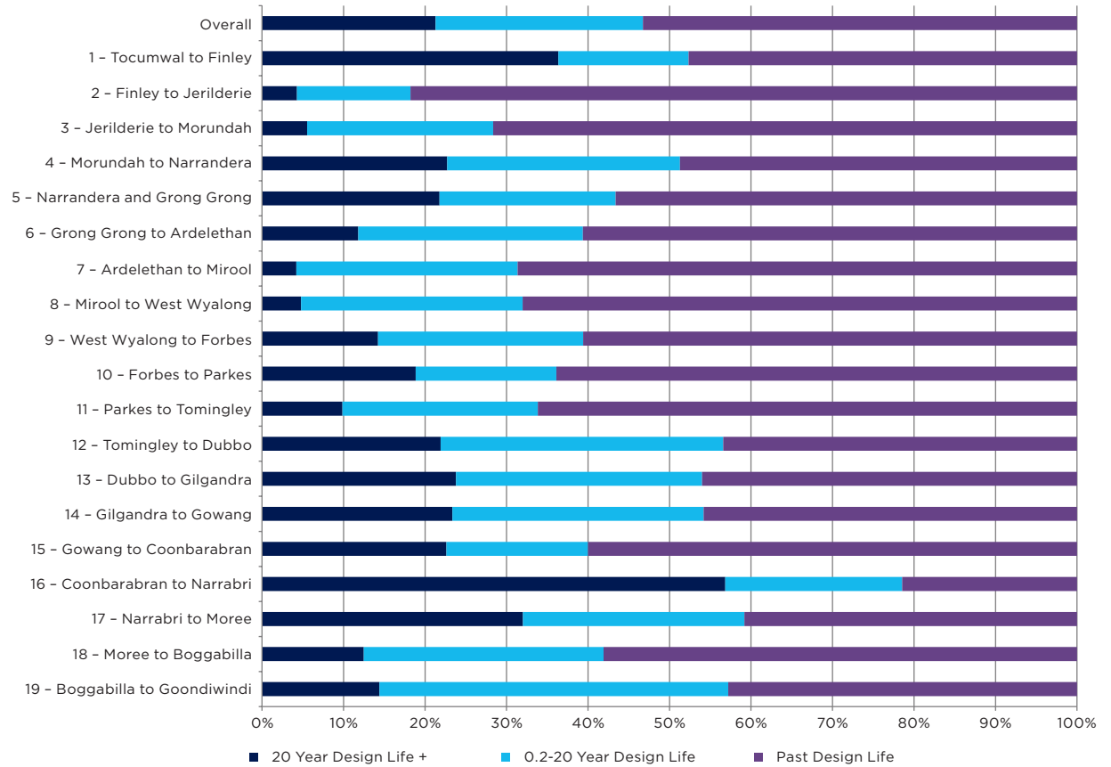
Figure 4.25 Curvature criteria
