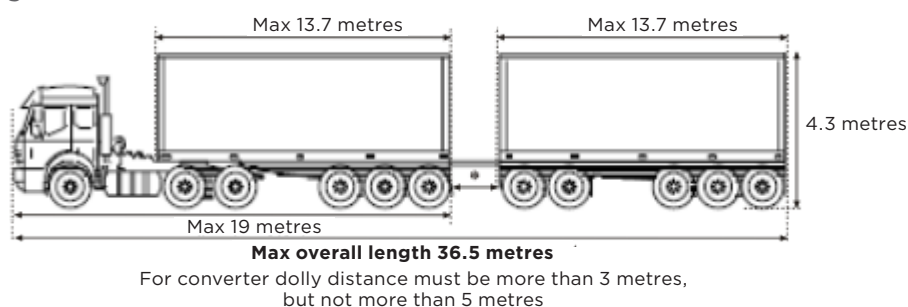
Figure 4.13 Double road train maximum dimensions
