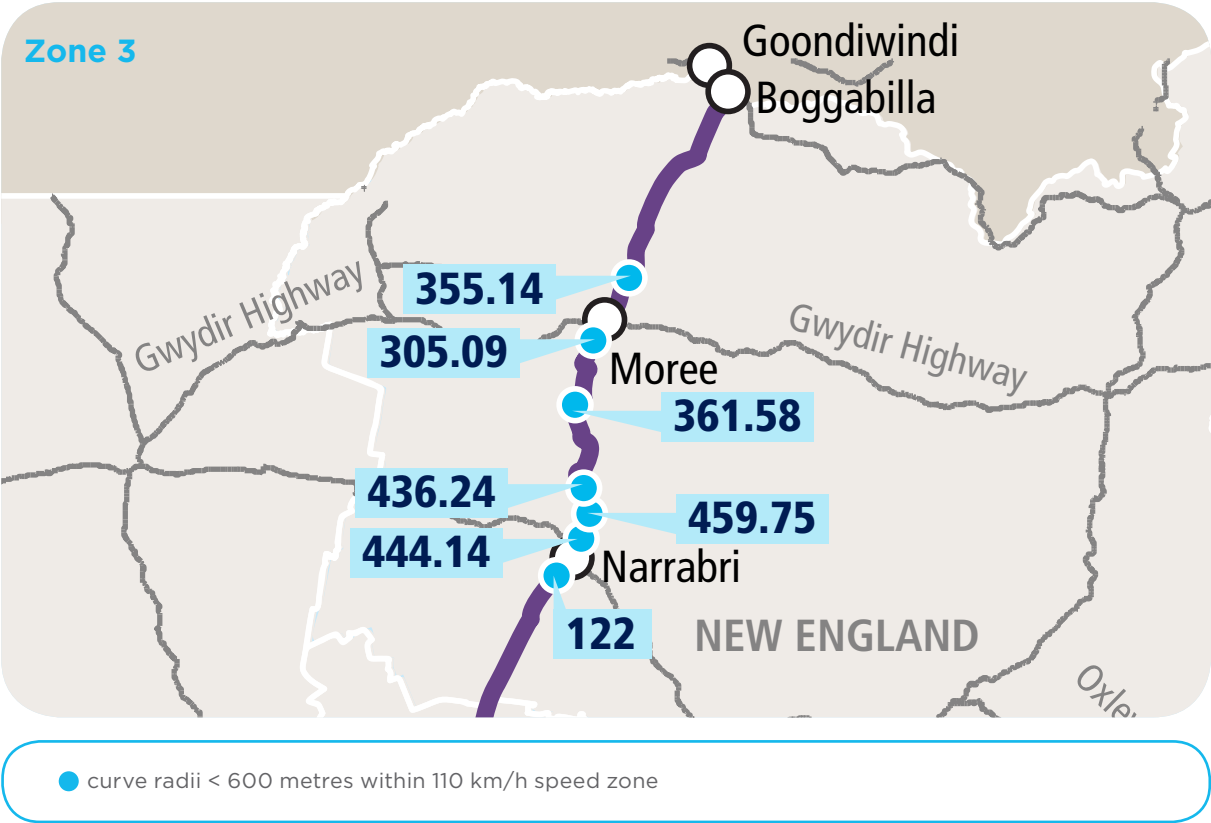
Figure 4.18 Locations where curve radii are less than 600 metres within 110 km/h speed zones (Zone 3)
