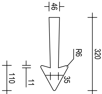
Symbol Detail
