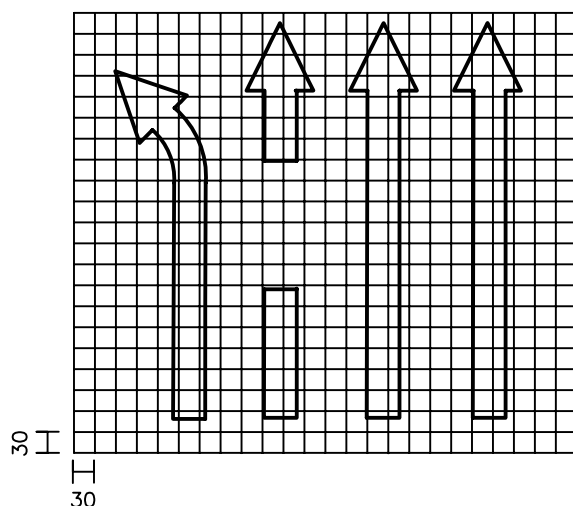
Symbol Detail
