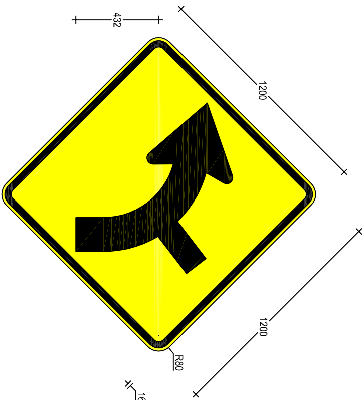
W2-9D(L) 1200 x 1200
