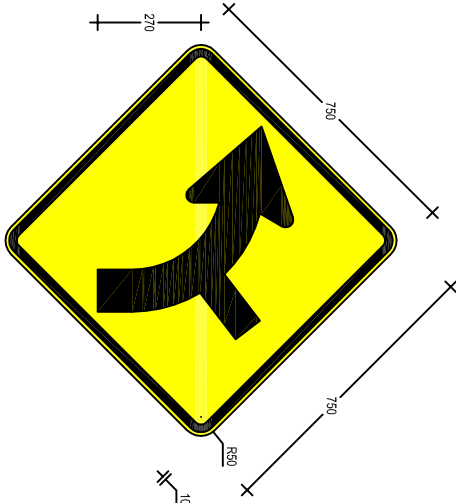
W2-9B(L) 750 x 750
