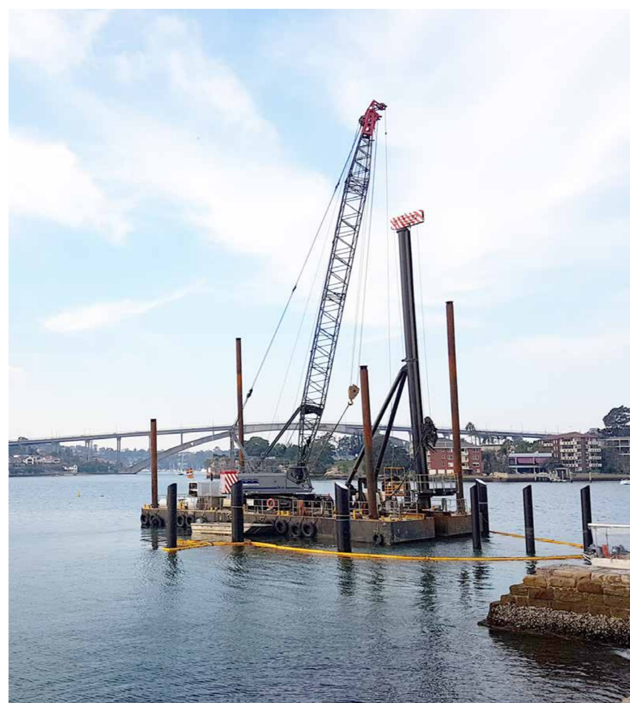
Barge-mounted crane at Chiswick
