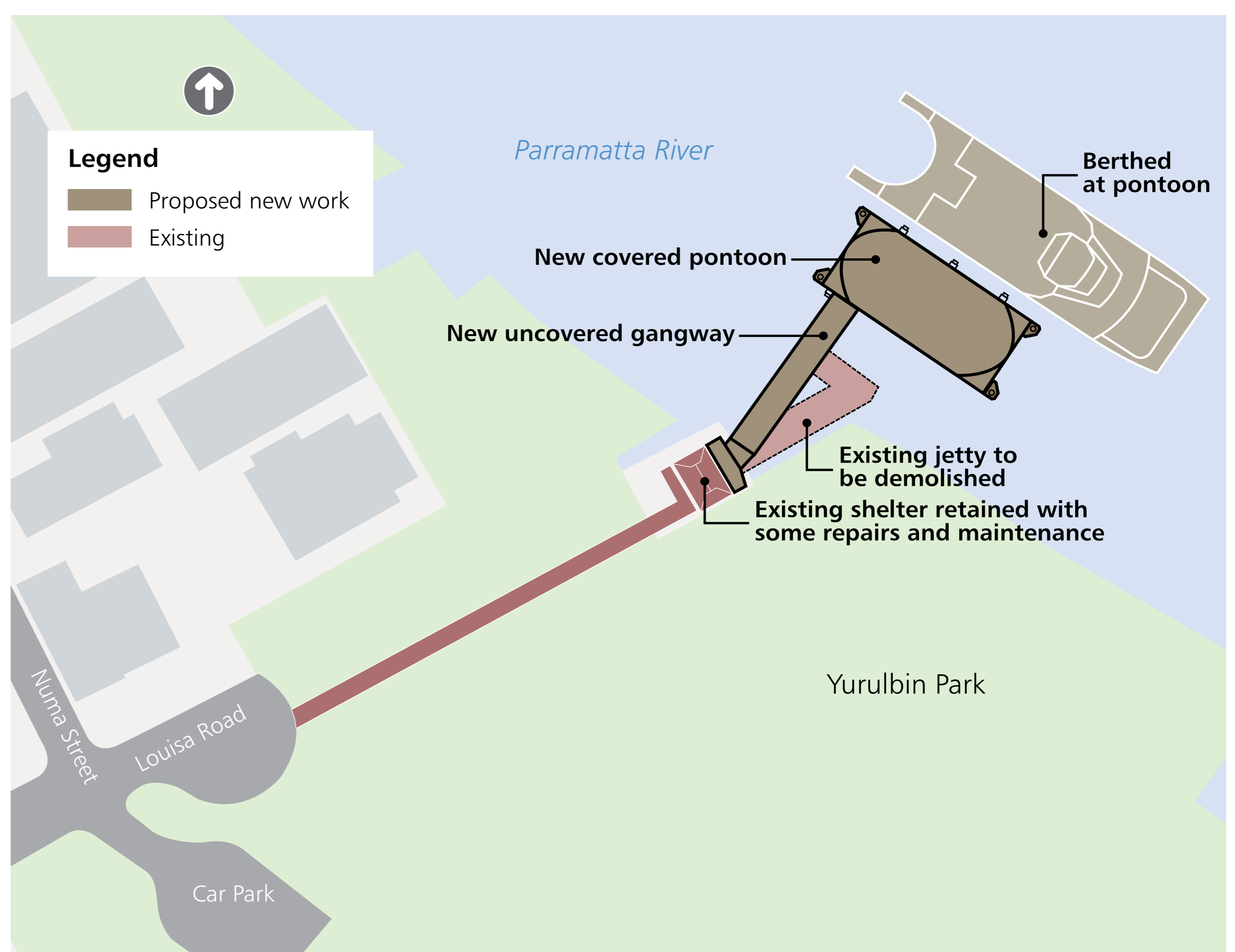
Proposed new wharf design for illustrative purposes
