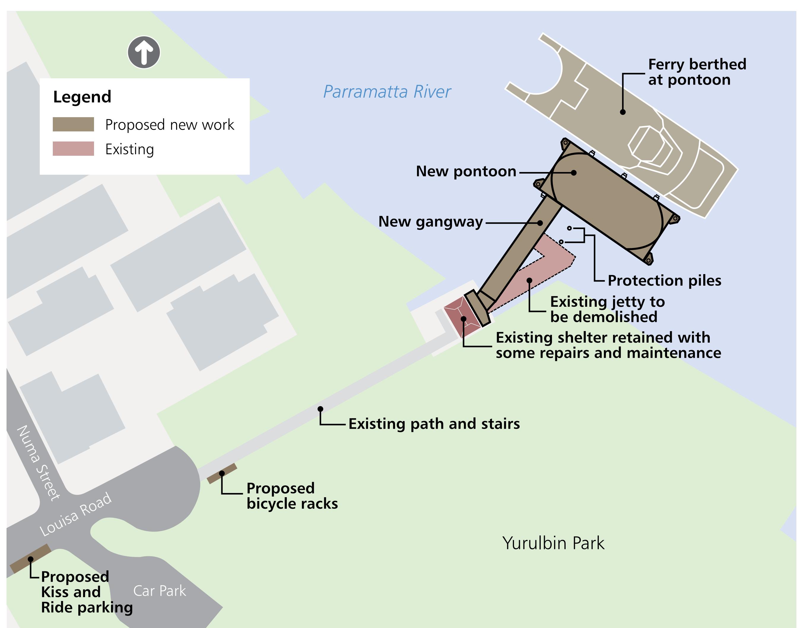
Proposed new wharf design for illustrative purposes
