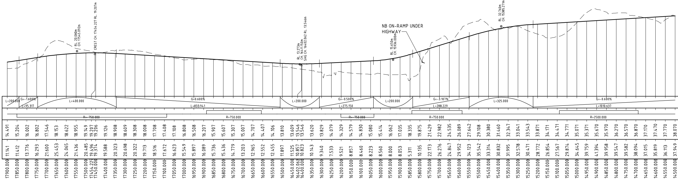
LONGITUDINAL SECTION ALONG CONTROL RMS HORIZONTAL SCALE 1:5000 VERTICAL SCALE 1:500
