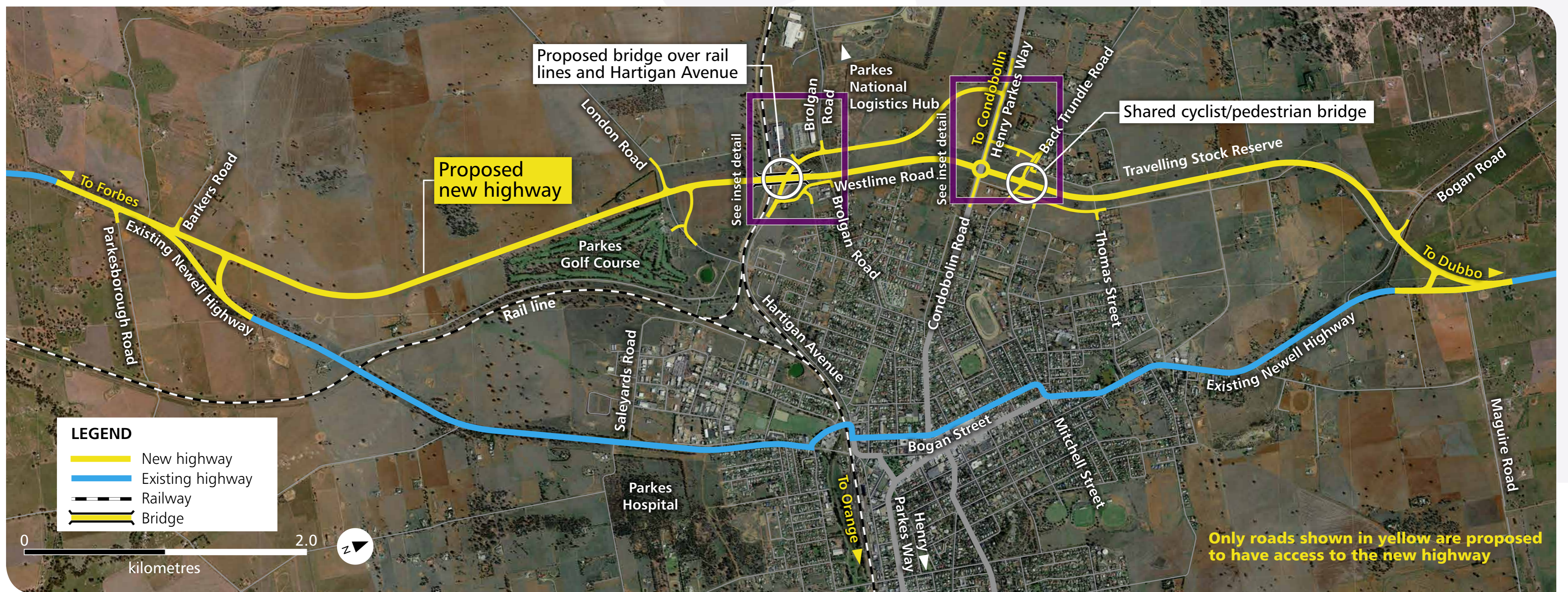
Concept design - Parkes Bypass
