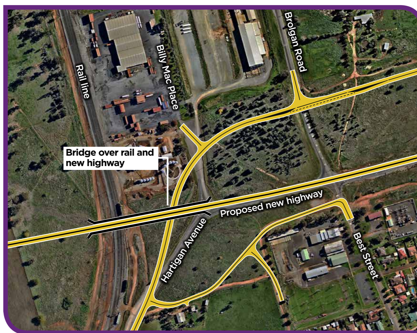
Inset detail: Bridge over Hartigan Avenue and the Broken Hill and Parkes to Narromine rail lines
