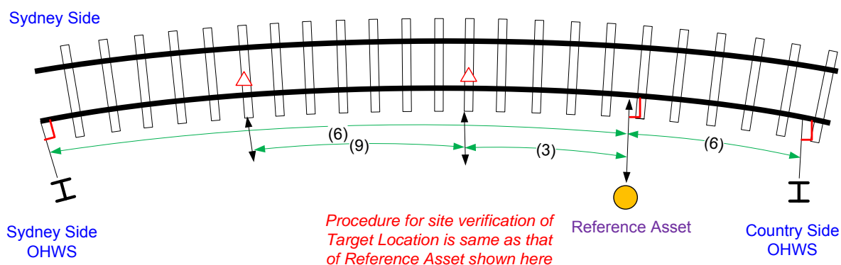
Figure 19: Measurement Procedure for AMS
