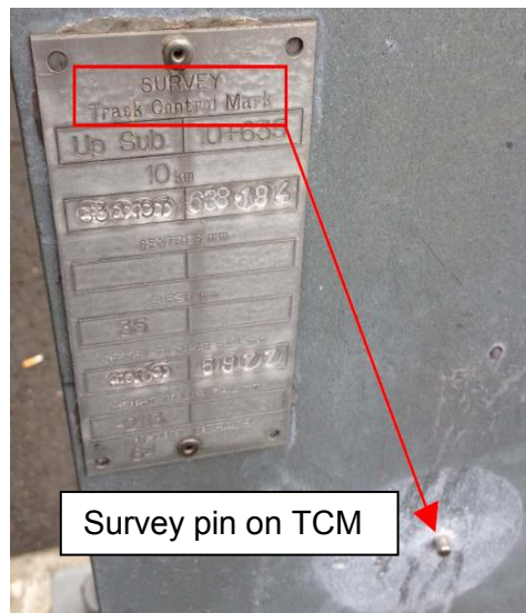
Figure 5: Survey pin located on an Overhead Wiring Structure
