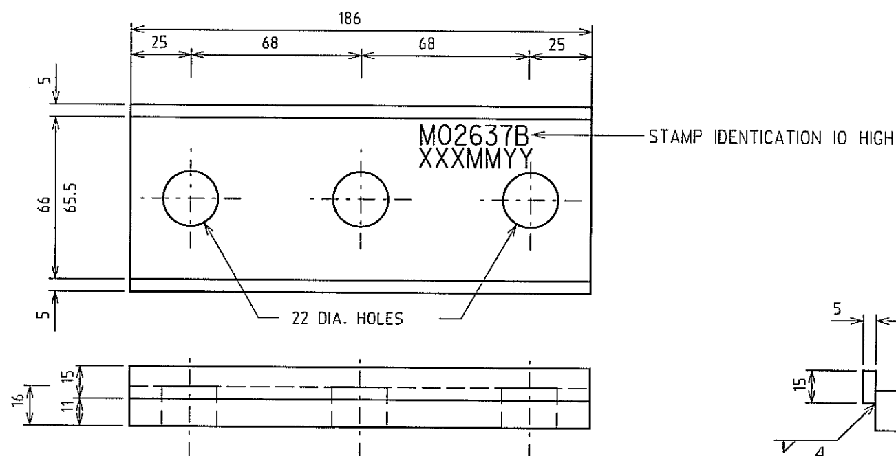
② DRIVE STRETCHER PACKING PIECE FOR 100mm SCARFING MATERIAL: STEEL TO AS3679-250, FINISH: 1 COAT OF R.O.Z.P. SUPPLY WITH THREE M20 X 90 Gr 4.6 ZINC PLATED HEX. HEAD BOLTS STOCK CODE 2062685
