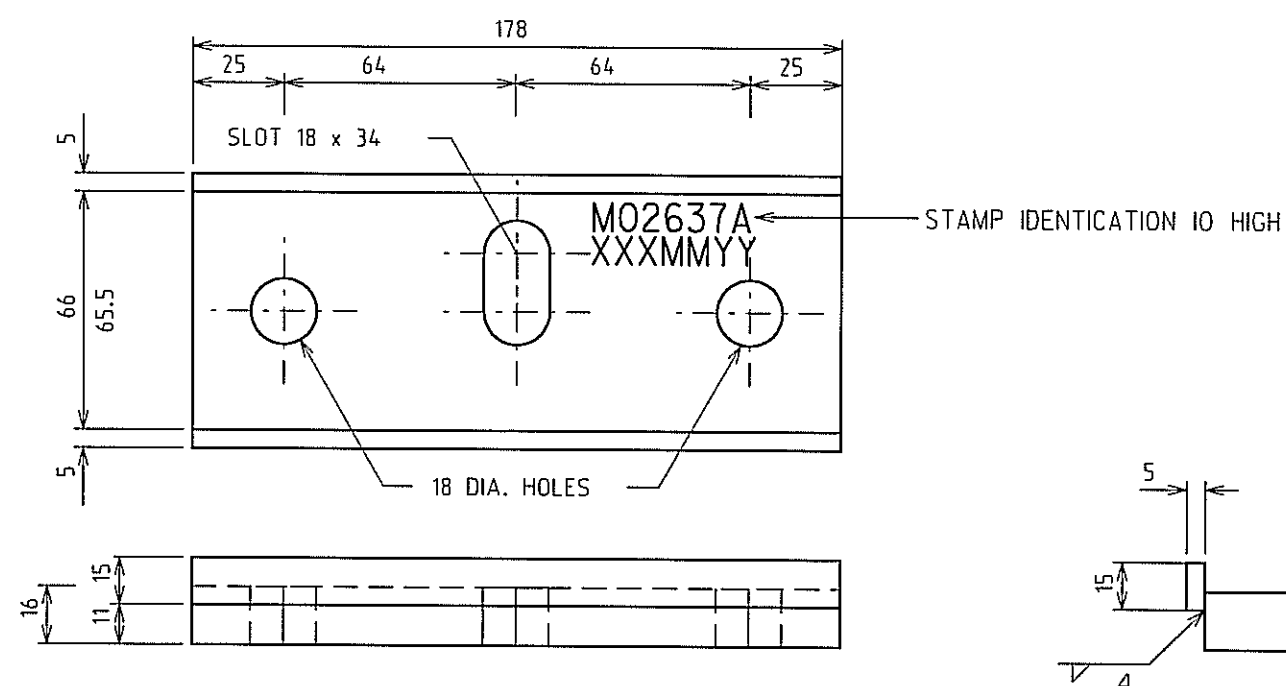
① LOCK STRETCHER PACKING PIECE FOR 100mm SCARFING MATERIAL: STEEL TO AS3679-250, FINISH: 1 COAT OF R.O.Z.P. SUPPLY WITH THREE M16 X 75 Gr 4.6 ZINC PLATED HEX. HEAD BOLTS STOCK CODE 2062677
