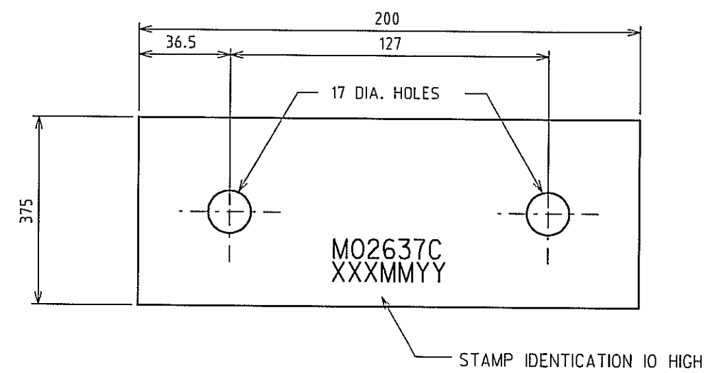
③ SWITCH MACHINE PACKING PIECE FOR 100mm SCARFING MATERIAL: NYLON OR TUFFCLAD 15 PLATE SUPPLY WITH TWO M16 X 100 LONG Gr 4.6 ZINC PLATED HEX. HEAD BOLTS STOCK CODE 2062693
