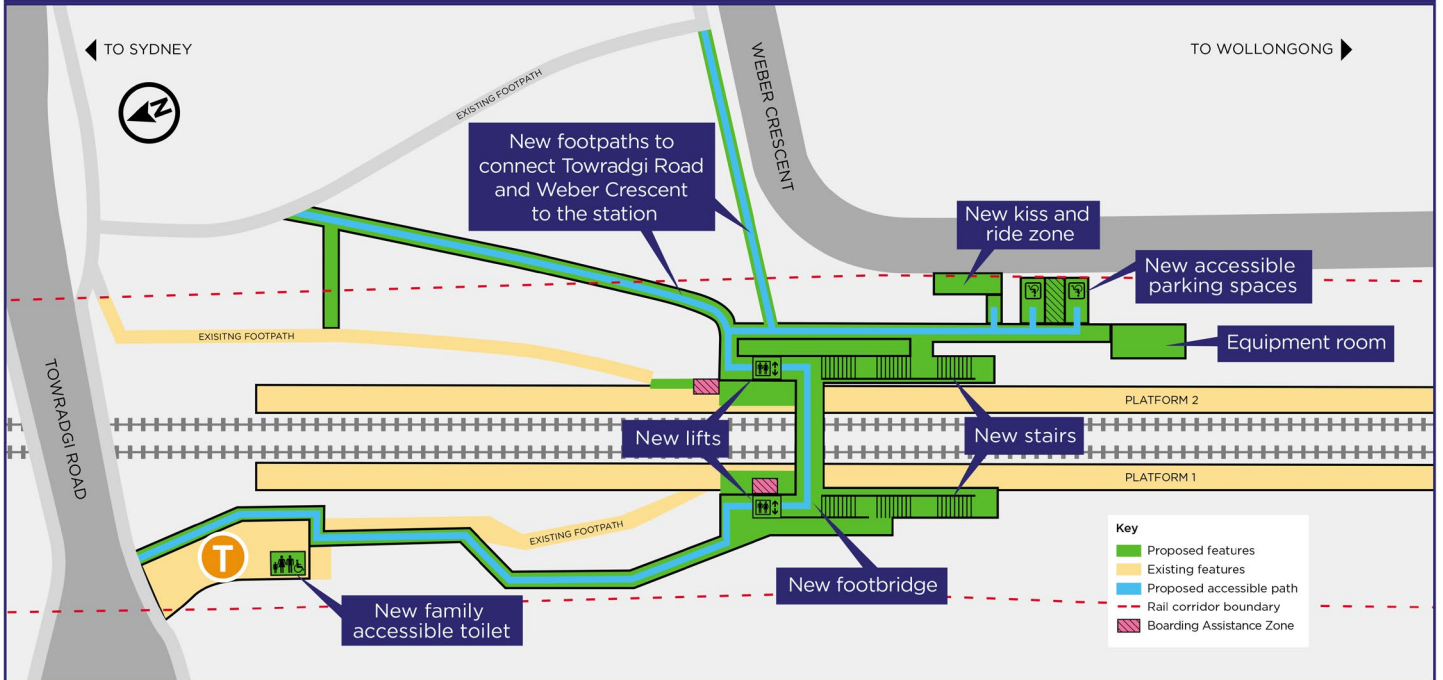
Key features of the proposed Towradgi Station Upgrade, subject to detailed design.
