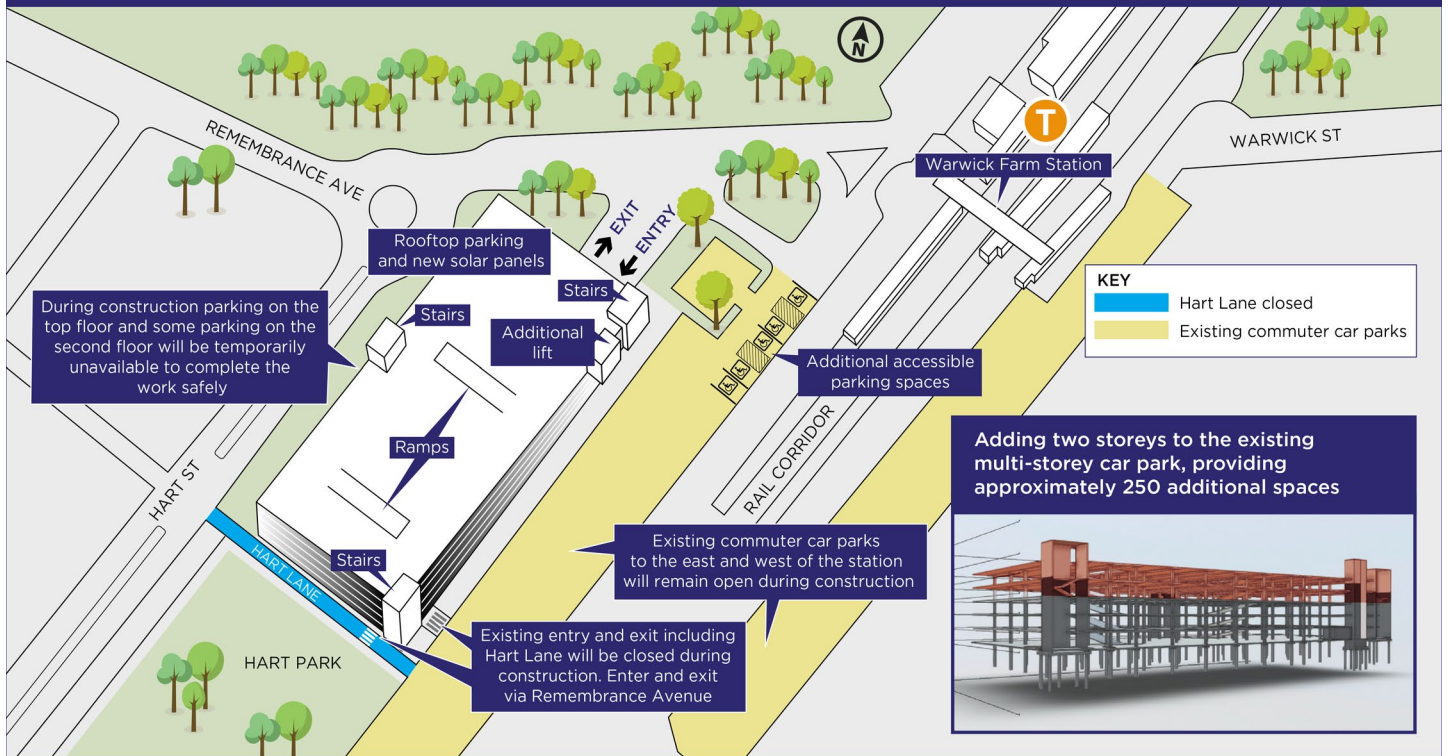
Site map of the commuter car park extension, subject to detailed design
