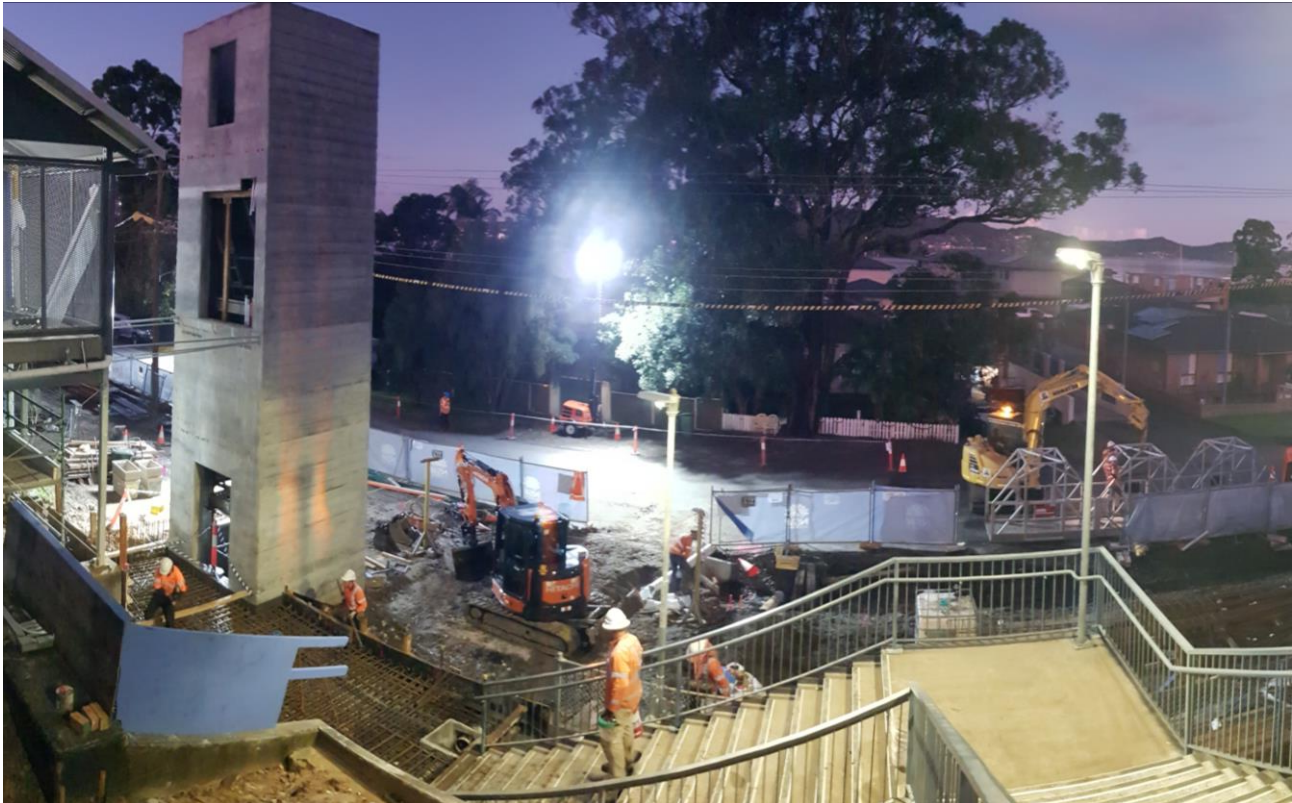
Station entry ready for concrete pour, and temporary ramp ready to be installed (by yellow mobile crane) at the Kurrawa Avenue side of Point Clare Station, late July 2022.
