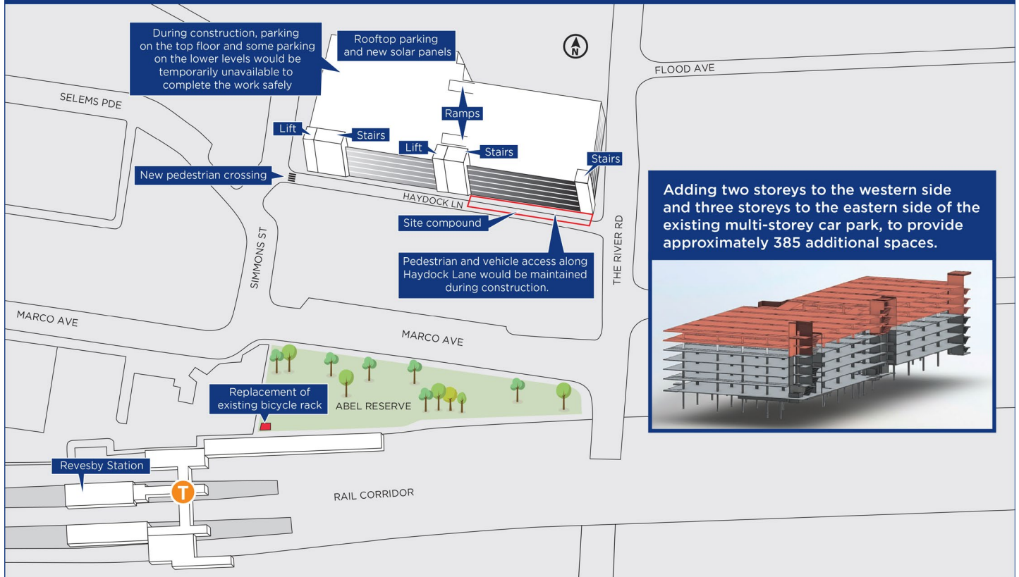
Site map of the new commuter car park, subject to planning approval and detailed design
