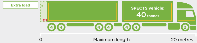
Performance Based Standards 3-axle truck and 4-axle dog trailer**
