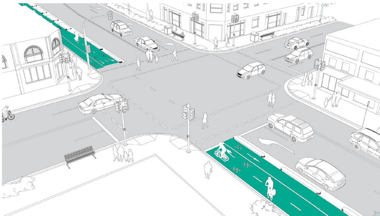
Figure 3.39 Bicycle path (two-way), signalised intersection - perspective
