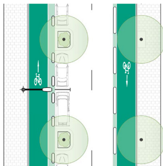
Figure 3.3 Typical plan - optimal configuration (unconstrained)
