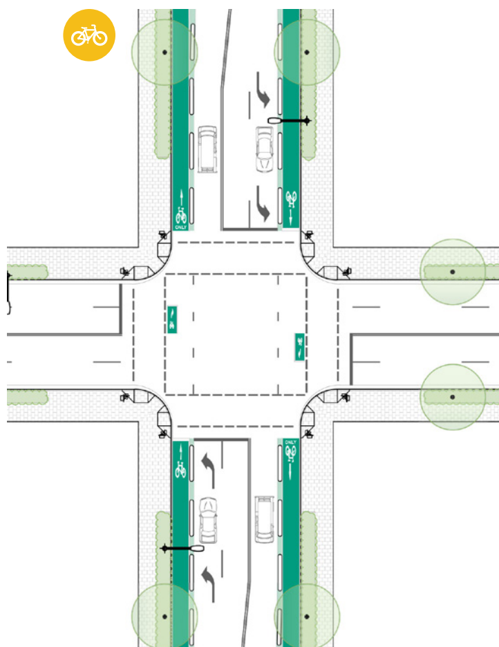
Figure 3.20 Bicycle path (one-way), signalised intersection - plan
