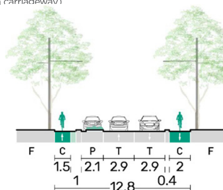
Figure 3.5 Typical cross section - constrained configuration (12.8m carriageway)
