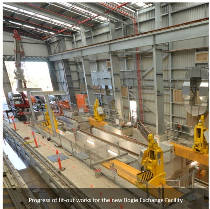
Installation of the Bogie drop tables in the underground chambers
