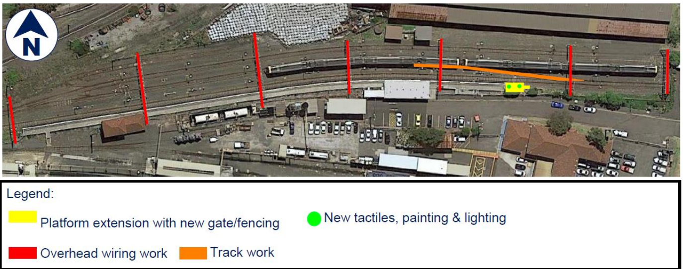
Overview image showing infrastructure improvements to be completed at Port Kembla Station
