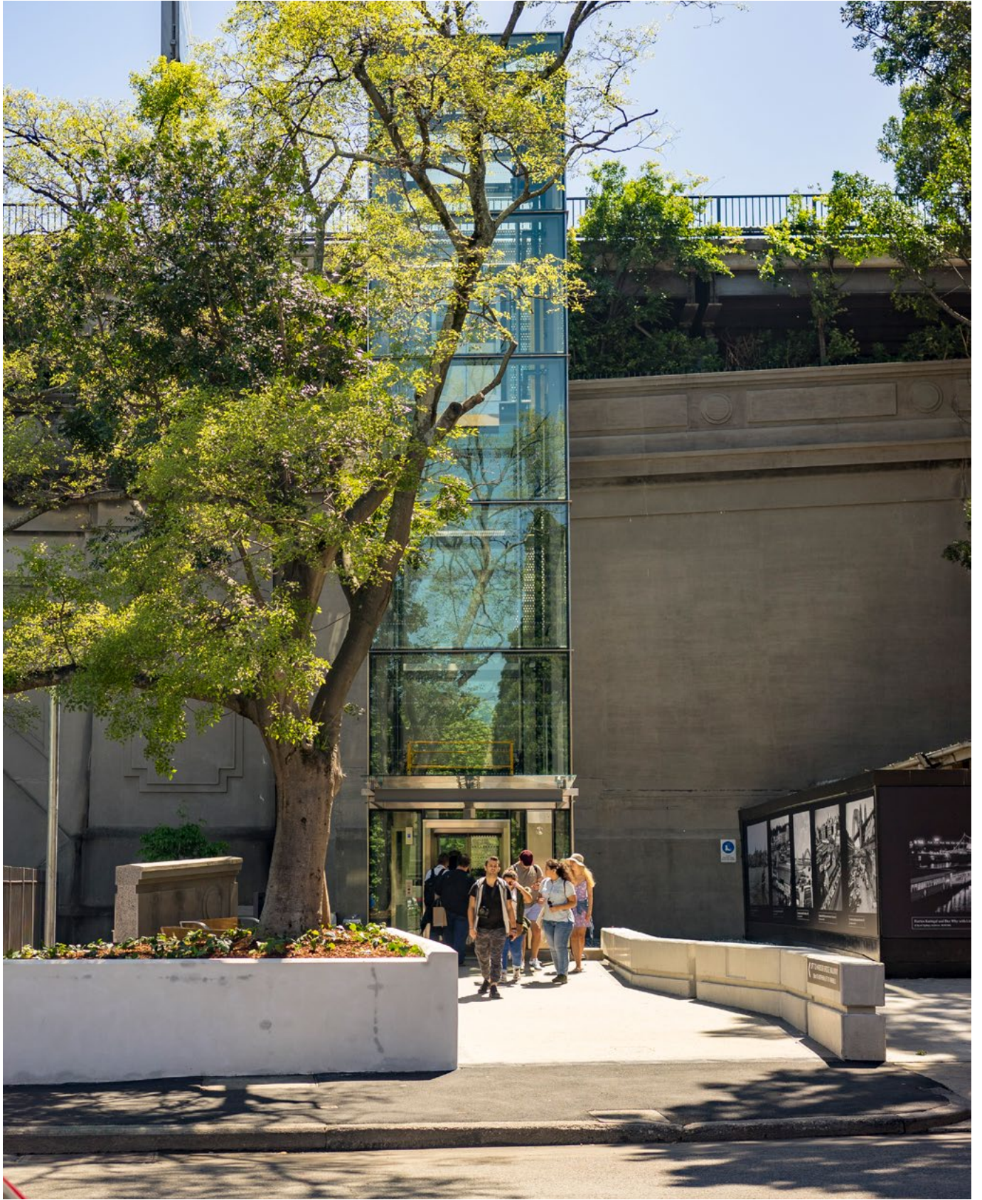
Lift access to the Sydney Harbour Bridge has been provided using modern materials, a simple refined design, and with minimal changes to the Sydney Harbour Bridge. The parapet removed for the southern lift has been used in the design of the access plaza.
