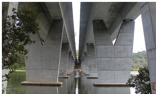
The bridges over the Georges River at Alford's Point utilise piers with a taper and triangular void. This 'Y' shaped pier is a refined and attractive way to support the two box girders.
