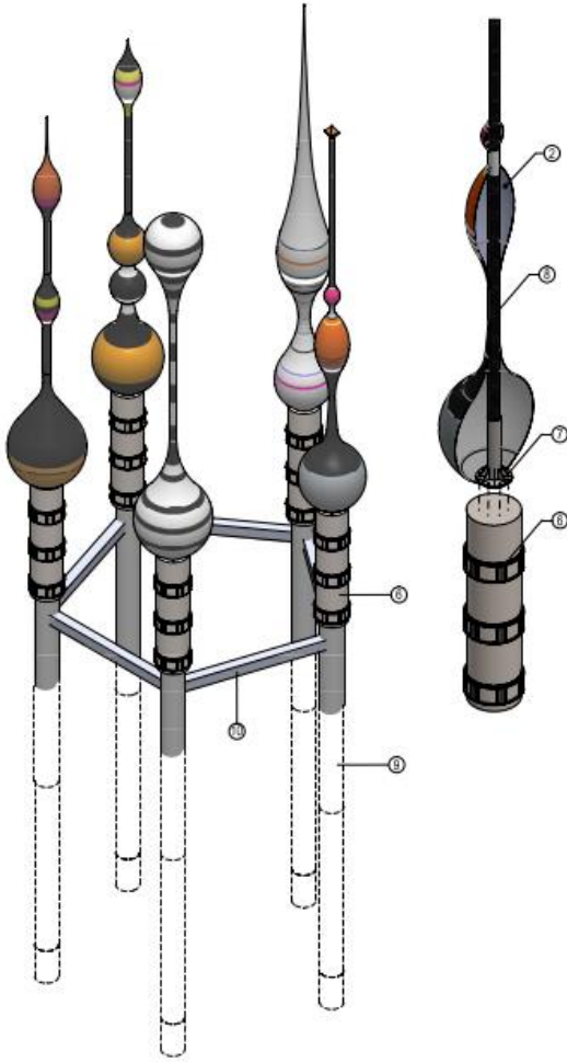
Isometric View
