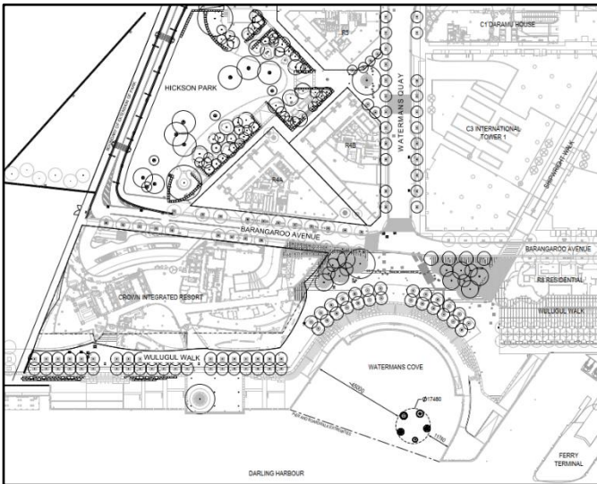
Site Plan
