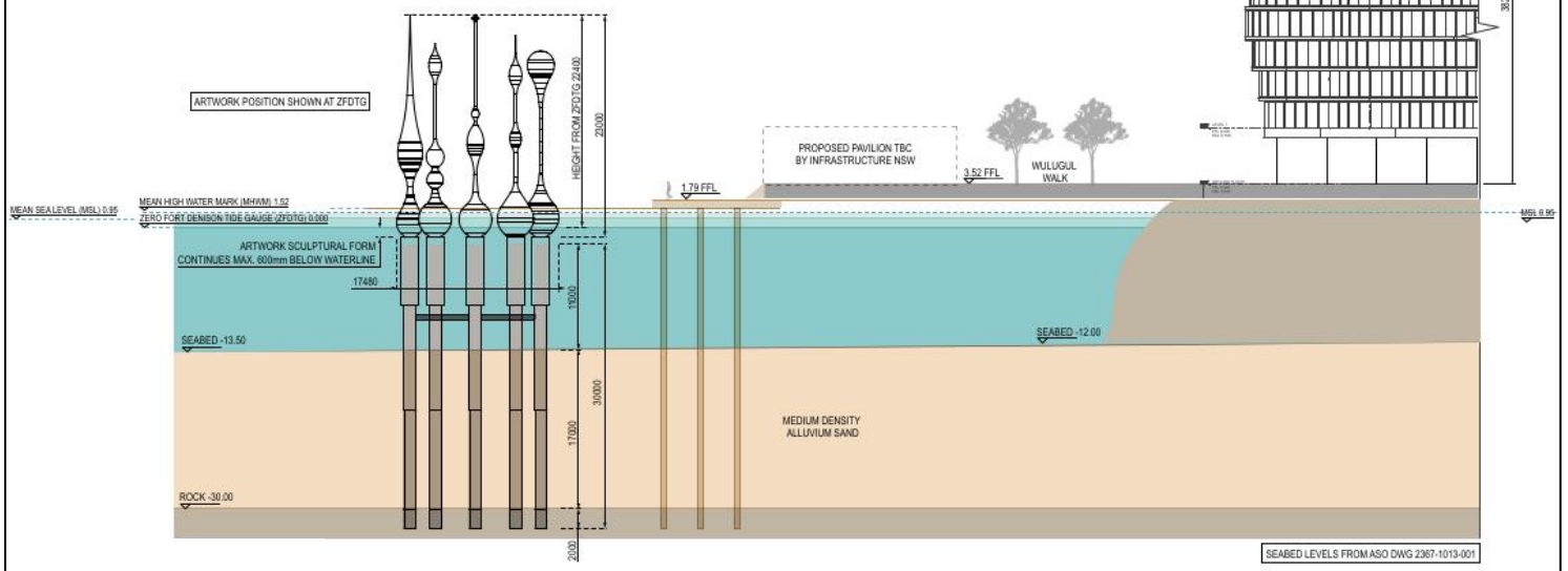
Section Plan
