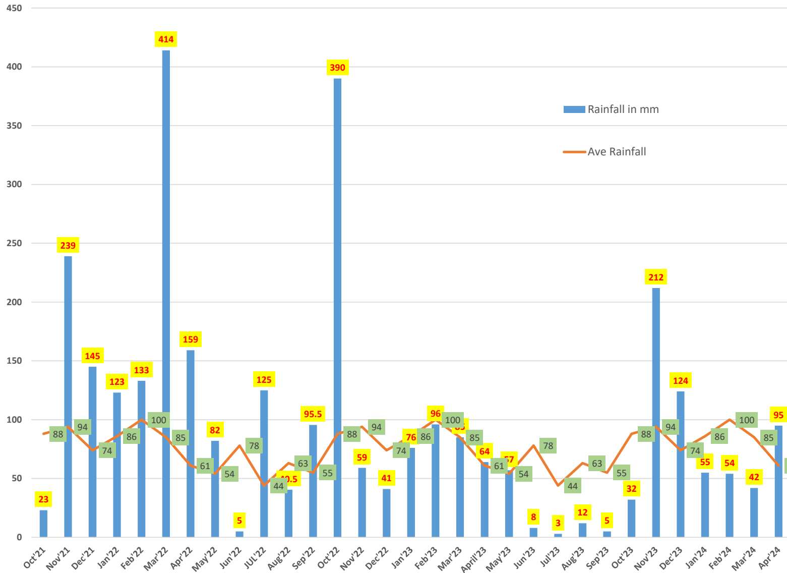
SBBLR - Monthly Vs Average Rainfall at Batemans Bay
