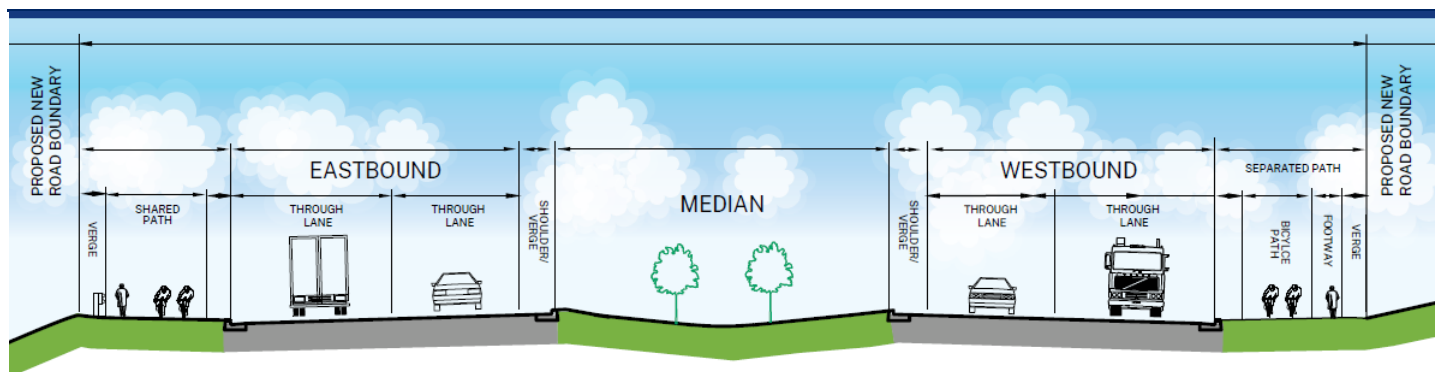
Concept design of the new proposed Southern Link Road
