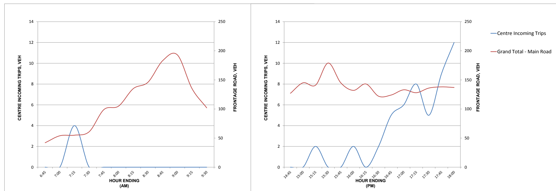
Figure 3.37 Site R2 WOOSH Care, Erina –15 Minute trip distribution – Vehicles – Tuesday 18/06/2015.
