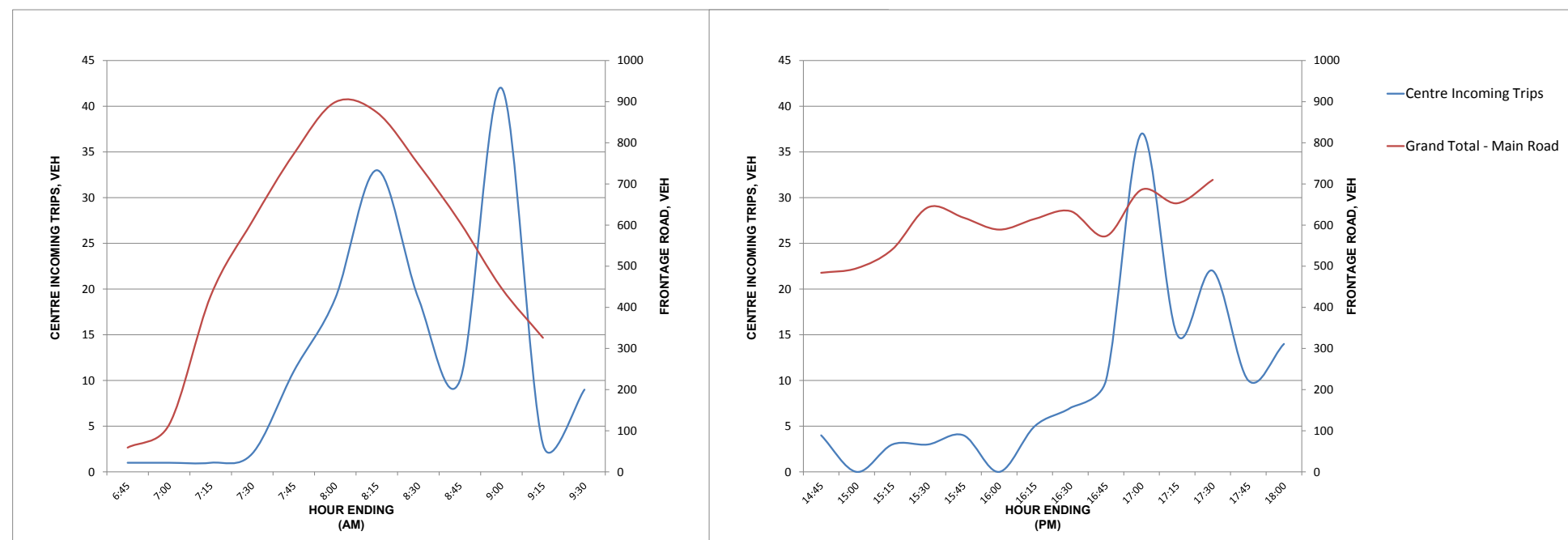
Figure 3.9 Site S4 Acre Woods Childcare, Roseville –15 Minute trip distribution – Vehicles – Tuesday 09/06/2015.
