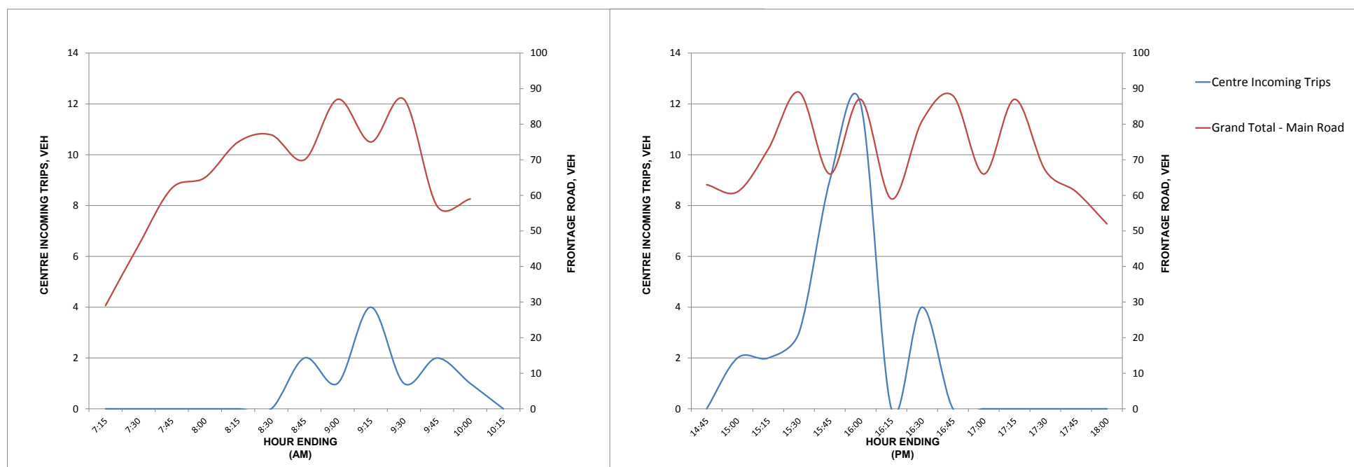
Figure 3.31 Site S11 Redfern Occasional Care, Redfern –15 Minute trip distribution – Vehicles – Thursday 18/06/2015.
