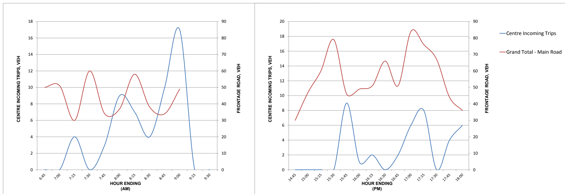
Figure 3.27 Site S9 YMCA Malabar OSHC, Malabar –15 Minute trip distribution – Vehicles – Wednesday 24/06/2015 (AM) - Thursday 25/06/2015 (PM).
