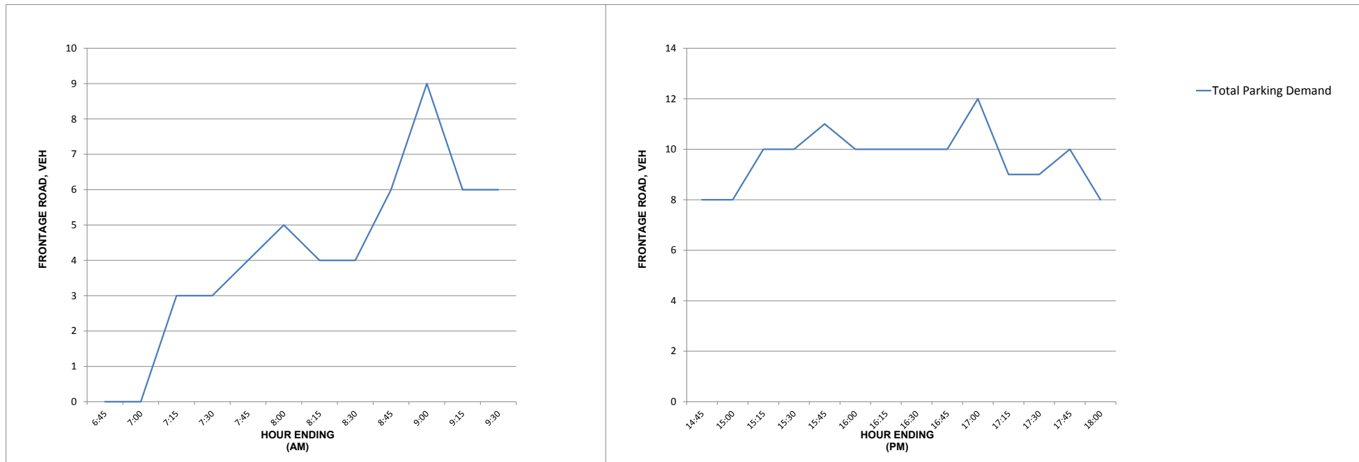
Figure 3.28 Site S9 YMCA Malabar OSHC, Malabar –15 Minute total parking demand – Vehicles – Wednesday 24/06/2015 (AM) - Thursday 25/06/2015 (PM).
