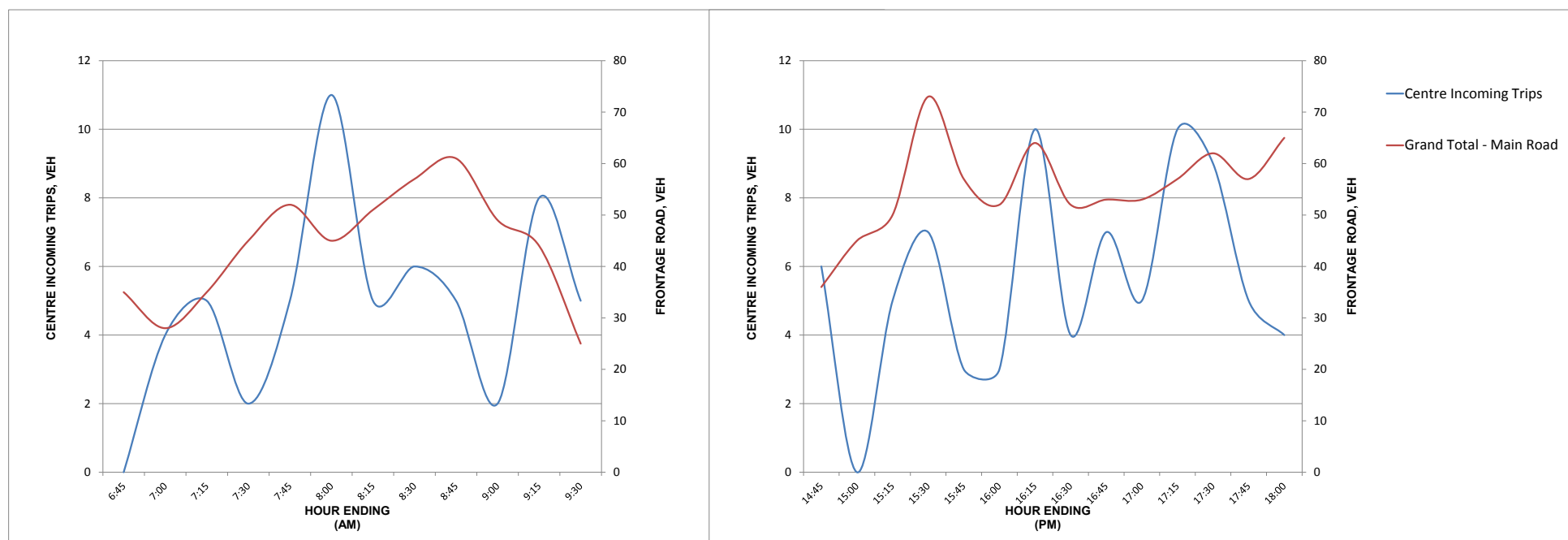
Figure 3.1 Site S1 Wattle Grove Long Day Care Centre, Wattle Grove –15 Minute trip distribution – Vehicles – Monday 01/06/2015.
