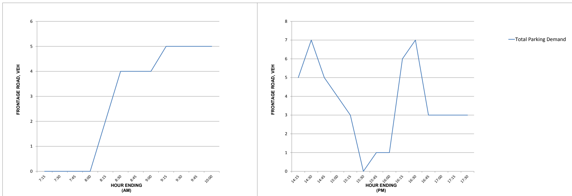
Figure 3.20 Site S5 Hilda Booler Kindergarten, Glebe –15 Minute total parking demand – Vehicles – Thursday 18/06/2015.
