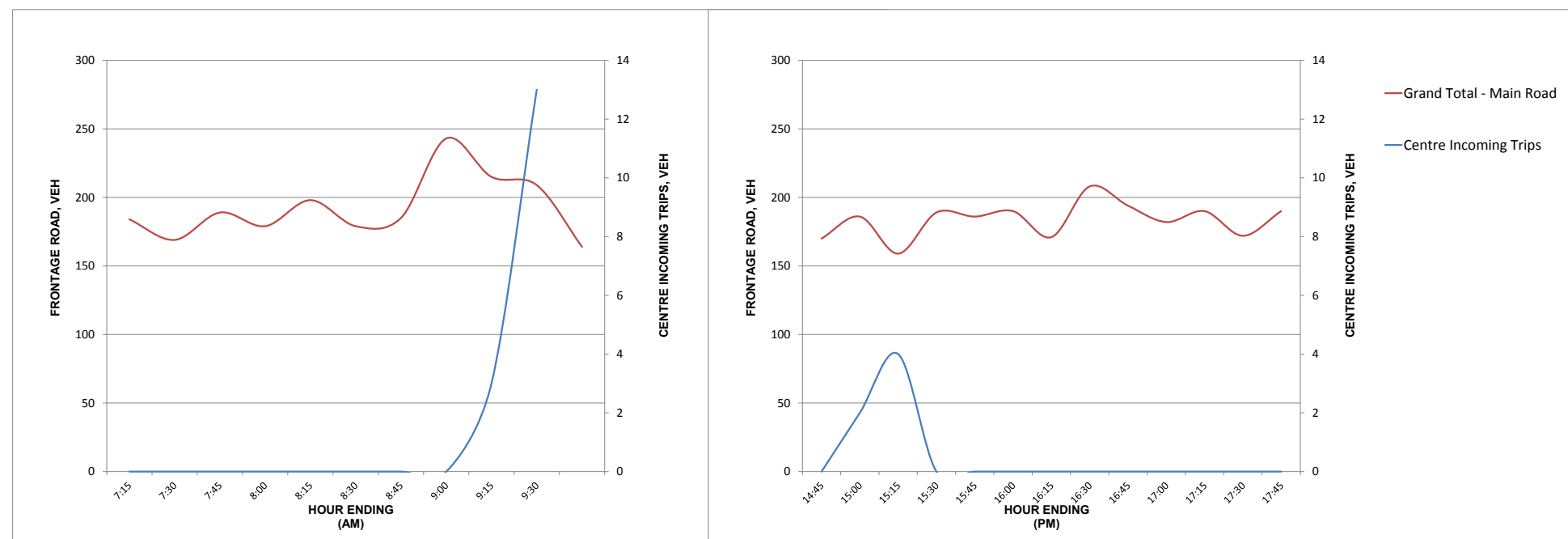
Figure 3.33 Site S12 Balmain/Rozelle Occasional Care, Balmain –15 Minute trip distribution – Vehicles – Monday 22/06/2015.
