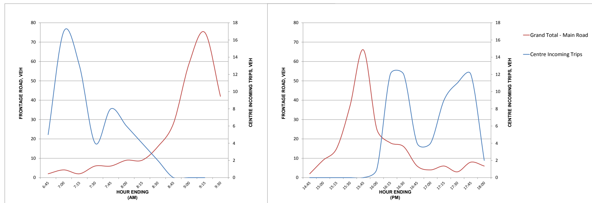
Figure 3.23 Site S7 Wattle Grove Public School OSHC, Wattle Grove –15 Minute trip distribution – Vehicles – Monday 01/06/2015.
