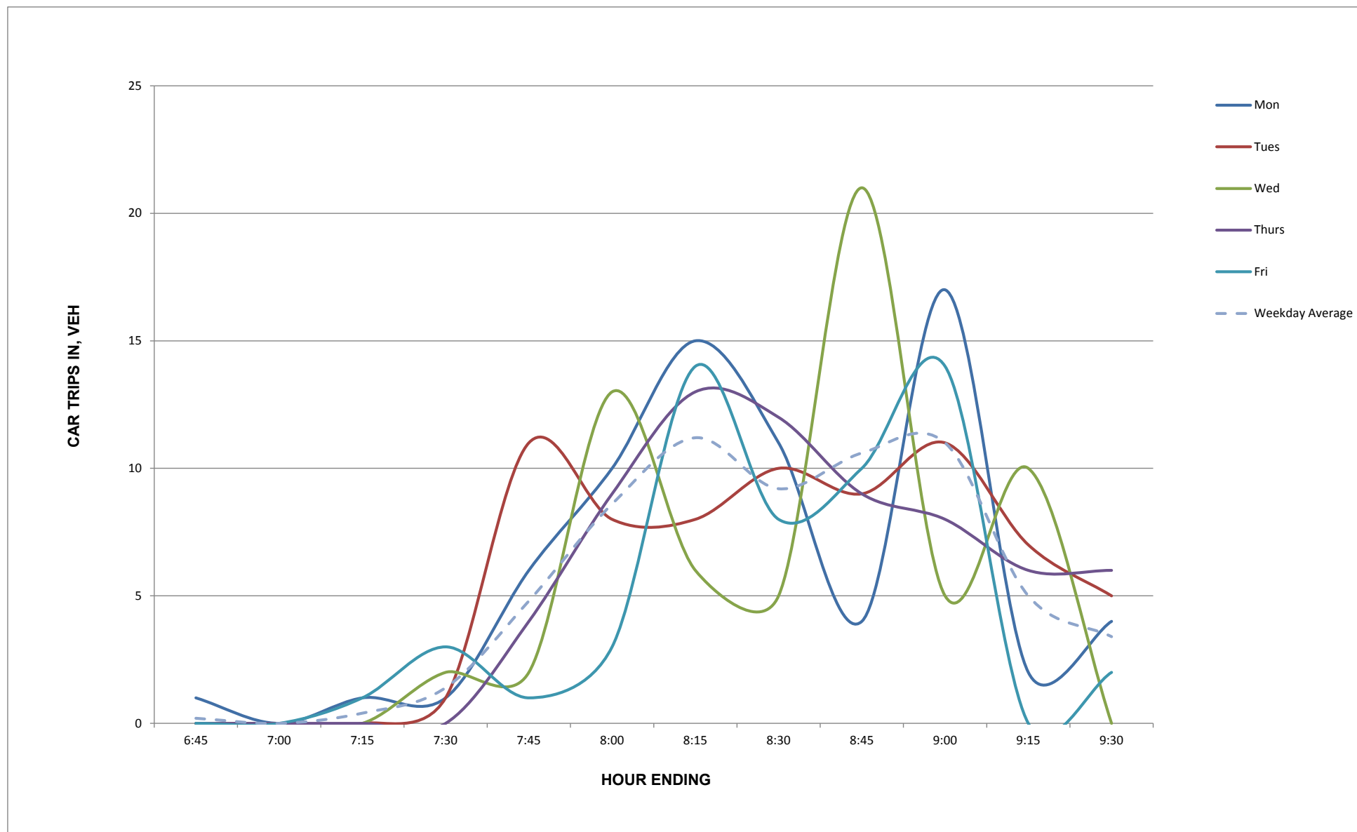
Figure 3.17 Site S4 Acre Woods Childcare, Roseville – 15 minute trip distribution AM – 5 days.
