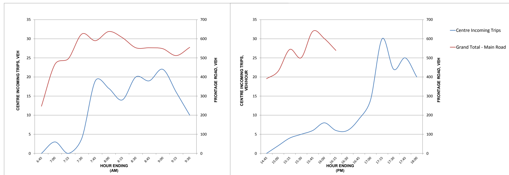
Figure 3.7 Site S4 Acre Woods Childcare, Roseville –15 Minute trip distribution – Vehicles – Monday 15/06/2015.
