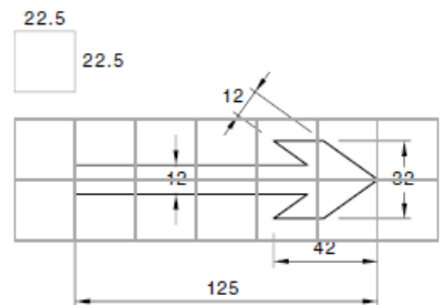
Symbol Detail (Not to scale)
