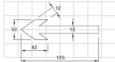
Symbol Detail (Not to scale)
